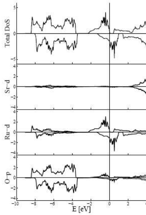
Figure 2.3: The total and partial density of state for \text{SrRuO}_3 [36].
