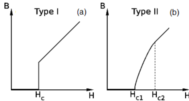
Figure 1.10: B vs H at type I (a) and type II (b) superconductors.
