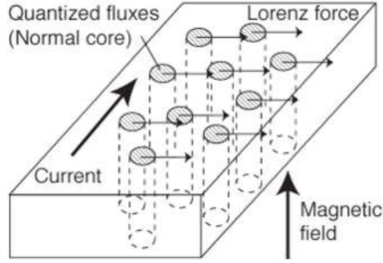
Figure 1.11: Lorentz force acting on the vortices, leads to their motion perpendicular to the current.
