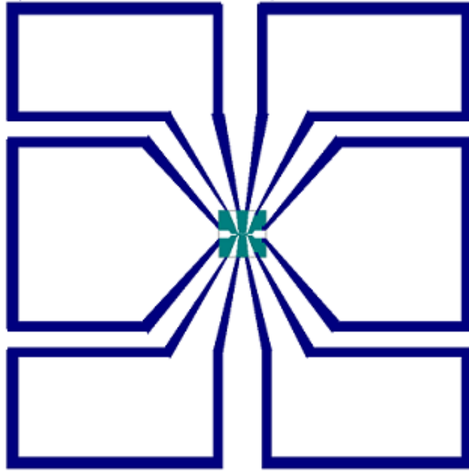
Figure 3.3: The patterning design of 1000 \times 1000 \text{ } ^1m . The colored lines show the area where \text{SrRuO}_3 was removed by etching.
