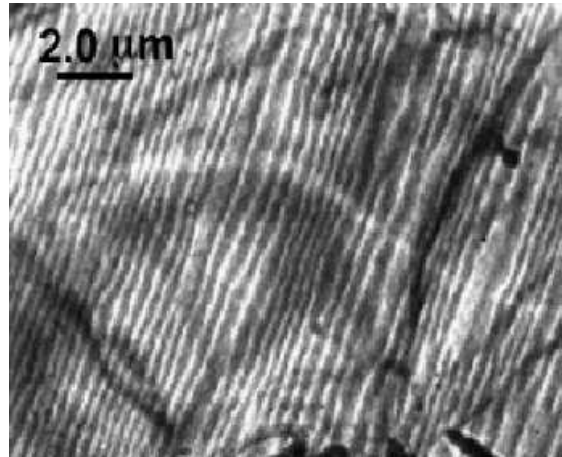
Figure 2.7: The TEM image of the narrow spaced DW's in the \text{SrRuO}_3 thin film grown on miscut \text{SrTiO}_3 substrate [37].
