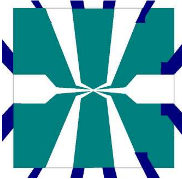
Figure 3.4: The patterning design of the "core" of the sample in the 100 \times 100 \mu m window. The colored area was removed by etching at the end of the processing.
